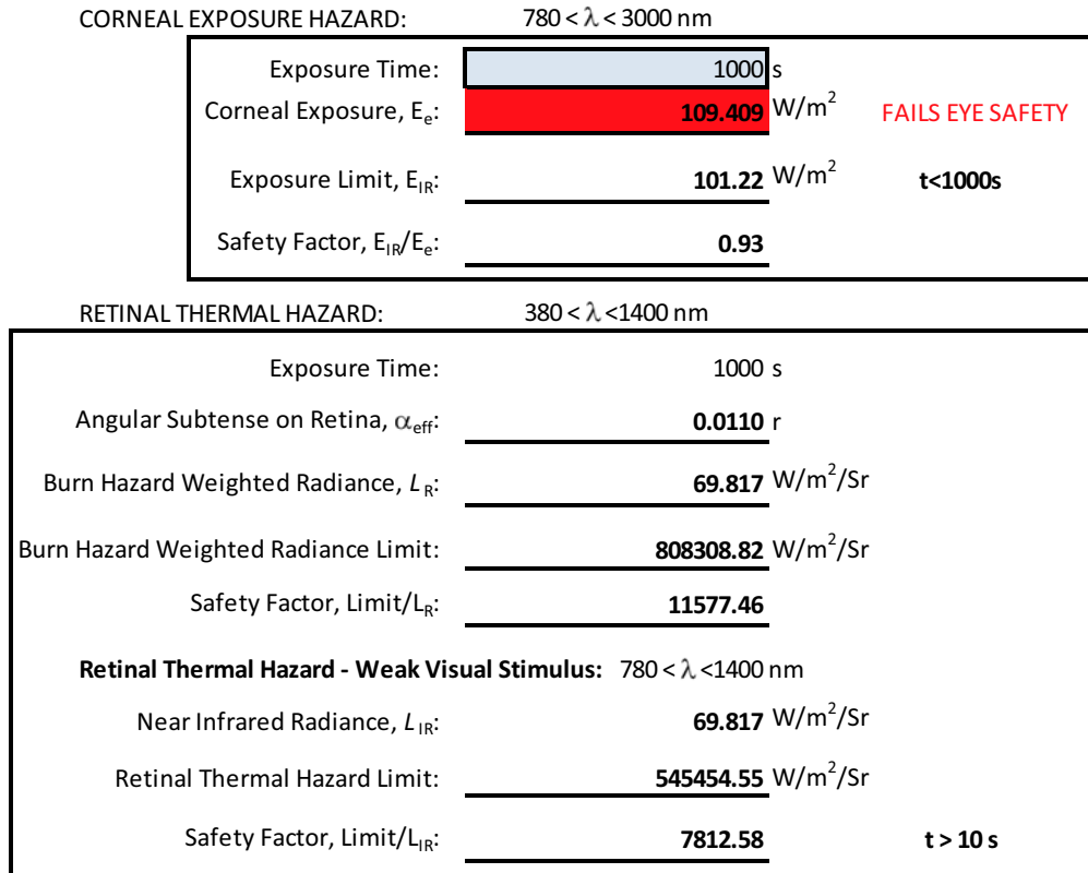
FIGURE 10. FAILING EYE SAFETY HAZARD CALCULATIONS
